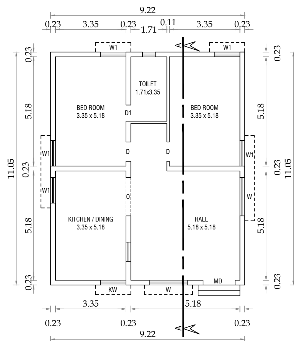
FLOOR PLAN
