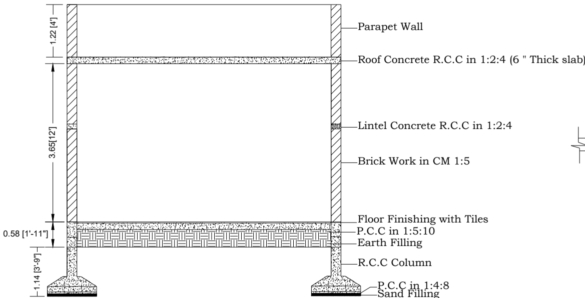
SECTION X-X
