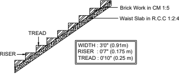
STAIRCASE DETAILS
