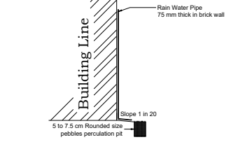
RAINWATER HARVESTING
