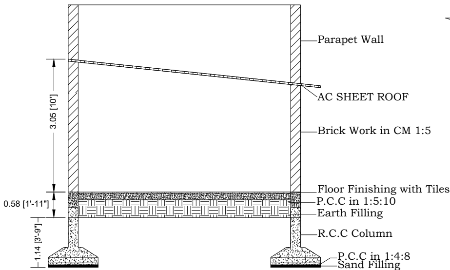
SECTION X-X
