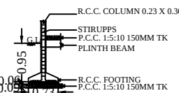
COLUMN DETAILS
