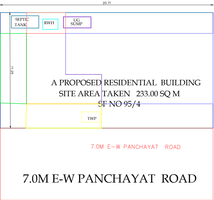
SITE PLAN
