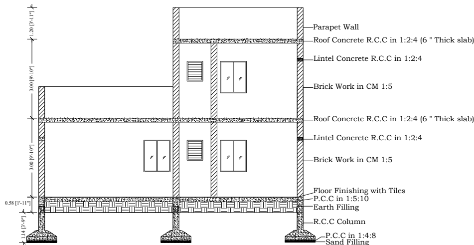
SECTION X-X
