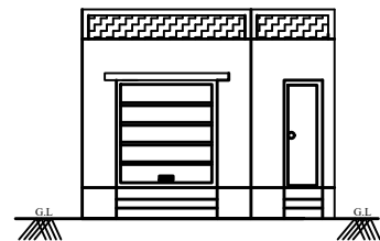
FRONT FACE ELEVATION
