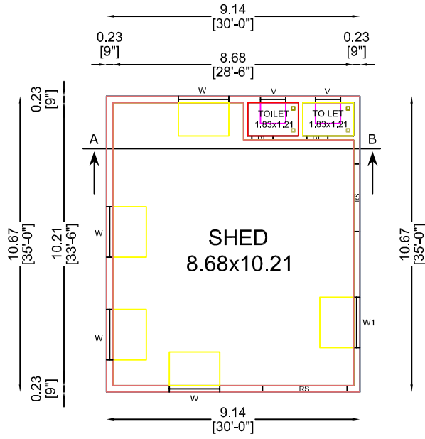
EAST FACE PLAN
