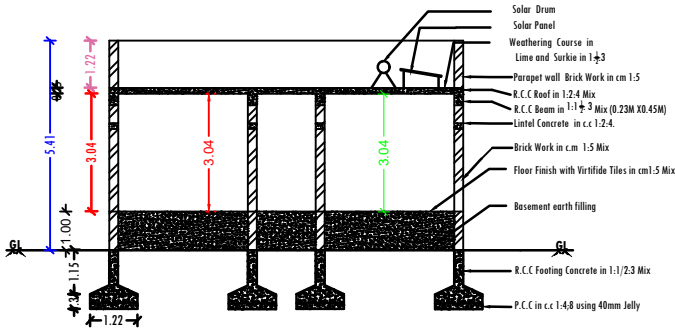
Section on "BC"
