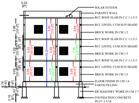
SECTION "AA","BB","CC"
