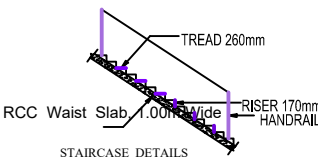
SECTION AHT
