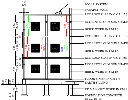
SECTION "AA","BB","CC"
