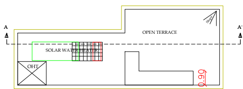
TERRACE FLOOR
