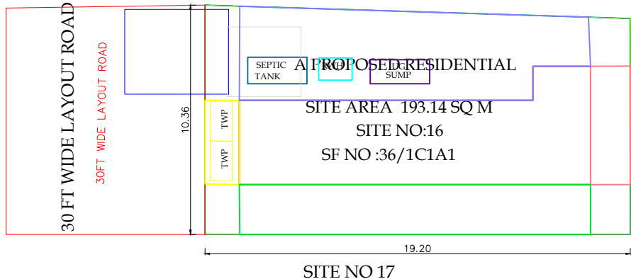
SITE PLAN
