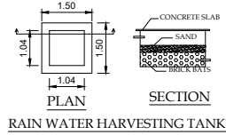
RAIN WATER HARVESTING TANK
