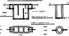
DETAILS OF SEPTIC TANK & SOAK PIT
