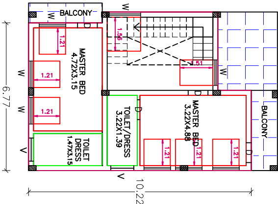
FIRST FLOOR PLAN (SCALE 1:100)
