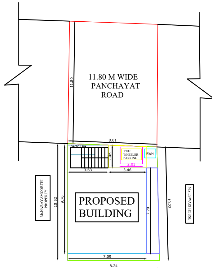
Mr.PALANISAMY, Mrs.SIVAKAMY HOUSE SITE PLAN
