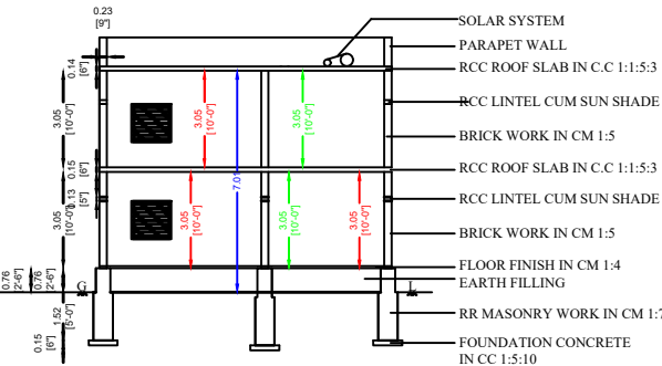
SECTION "AA","BB"
