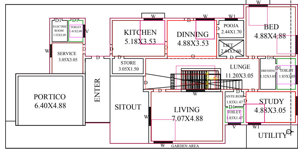
PROPOSED.GF.PLAN
