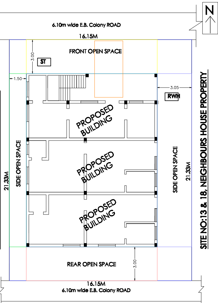
DETAILED SITE PLAN SCALE 1:100
