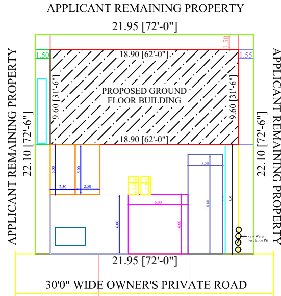
SITE PLAN
