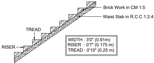
STAIRCASE DETAILS
