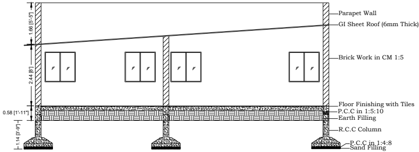
SECTION X-X
