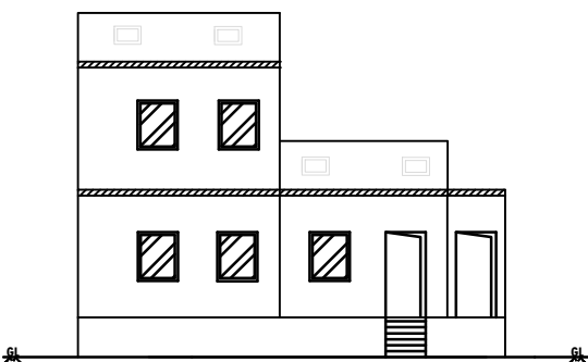
Elevation on "A"
