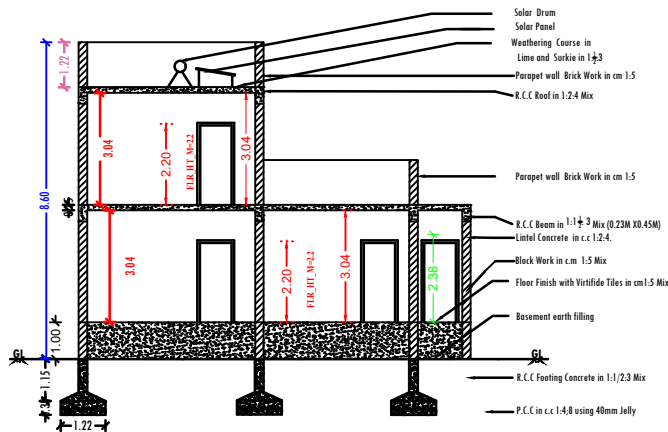
Section on "BC"
