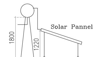
SIDE ELEVATION (Not to scale)
