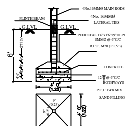
FOUNDATION DETAIL
