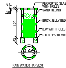
RAIN WATER HARVEST
