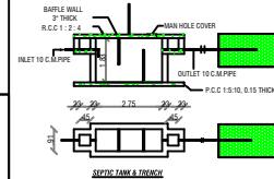
SEPTIC TANK & TRENCH
