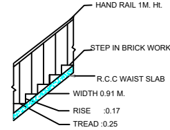
STAIR DETAIL
