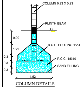
COLUMN DETAILS
