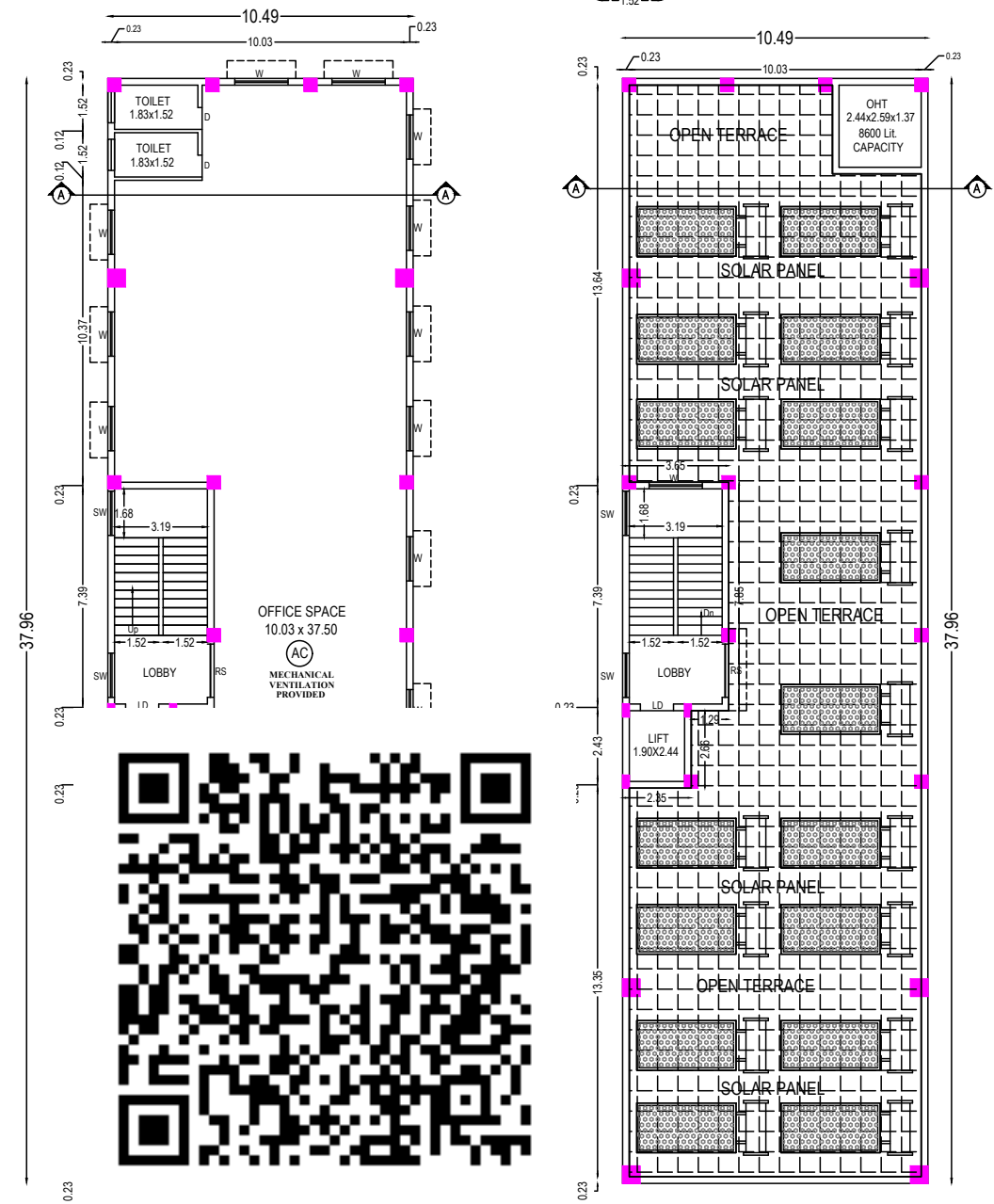
TYPICAL FLOOR ( FIRST, SECOND AND THIRD FLOOR PLAN)
