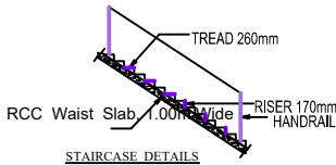
STAIRCASE DETAILS
