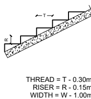
STAIRCASE DETAILS
