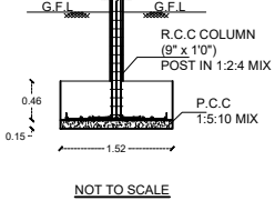
COLUMN POST DETAILS
