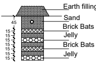
SECTION ON B-B.
