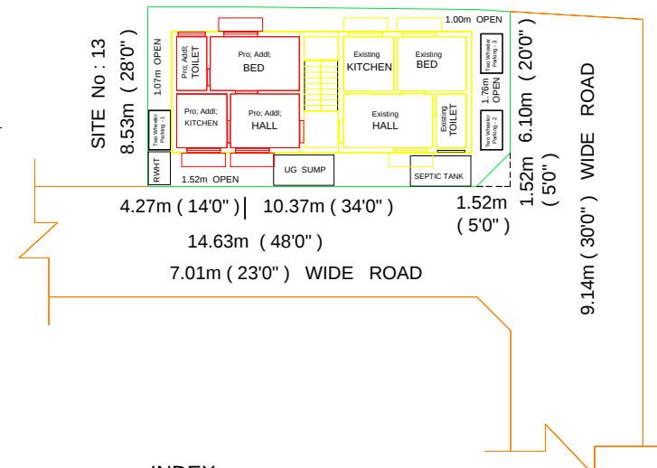
FIRST FLOOR PLAN (ALREADY APPROVED - IN PART OF EXISTING AND IN PART OF PROPOSED ADDITIONAL)
