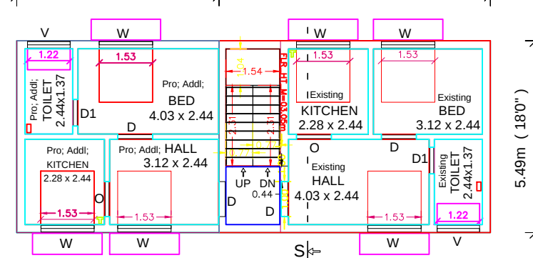
FIRST FLOOR PLAN (ALREADY APPROVED - IN PART OF EXISTING AND IN PART OF PROPOSED ADDITIONAL)
