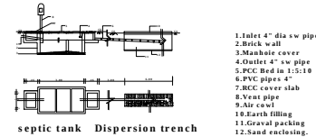
KEY MAP SEPTIC TANK DETAILS
