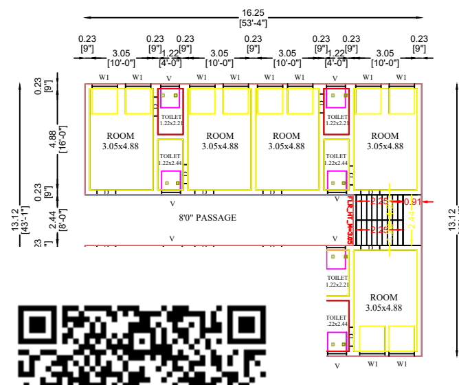
R PLAN
