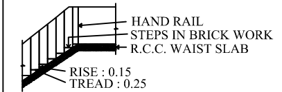
STAIR DETAILS
