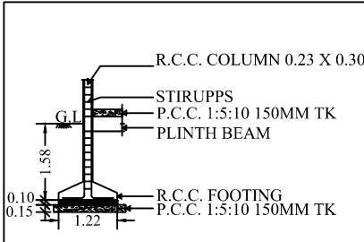
COLUMN DETAILS
