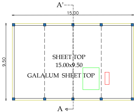
TERRACE FLOOR
