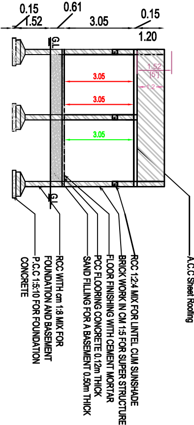
SECTION -AA
