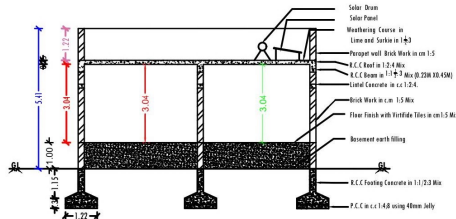
Section on "BC"
