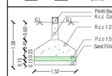
COLUMN FOOTING DETAILS
