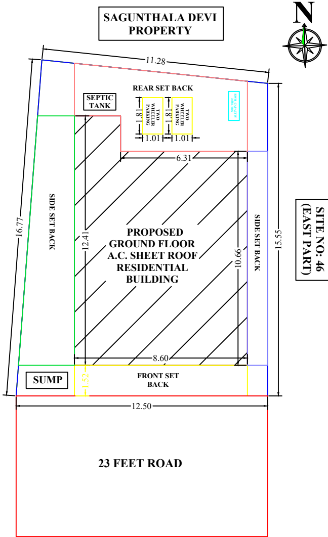
SITE PLAN
