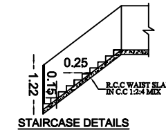
STAIRCASE DETAILS
