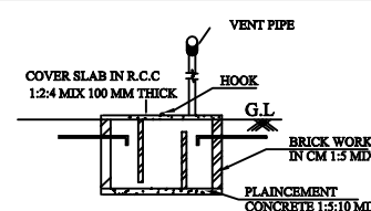
DISPERSION TRENCH
