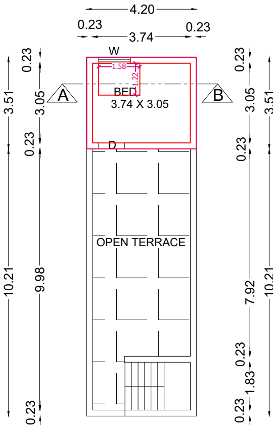
FRIST FLOOR PLAN
