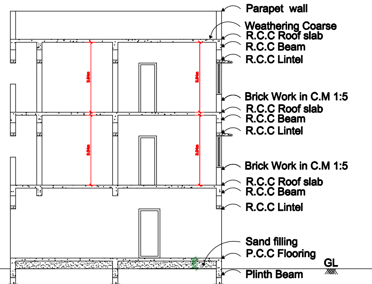
SECTION ON "RR"
