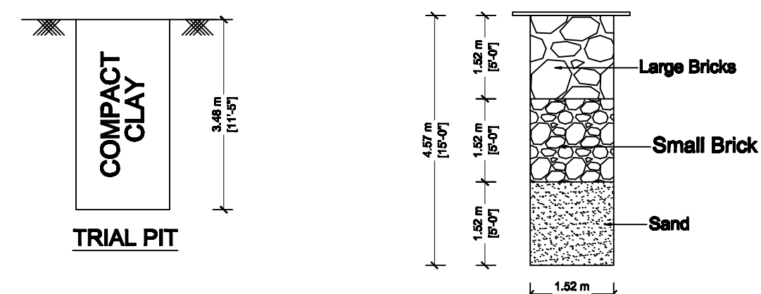
SECTION OF RAIN WATER COLLECTION PITS (NTS)
