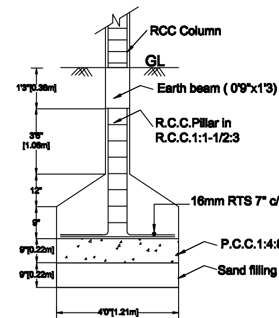
FOUNDATION DETAILS
