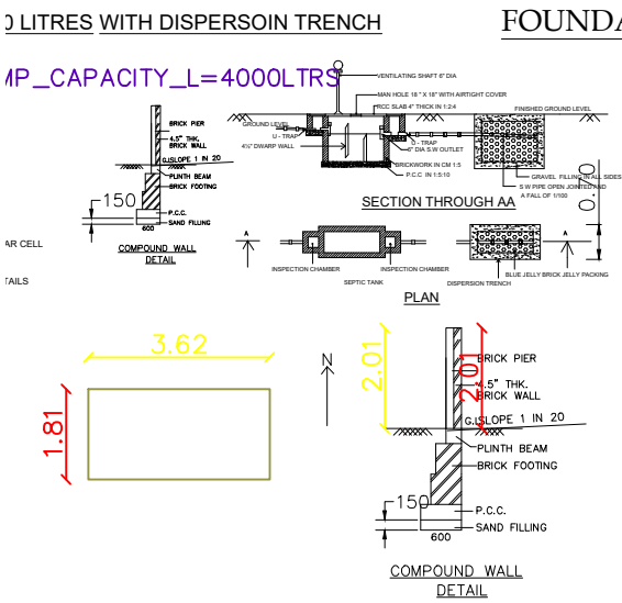
FOUNDATION DETAIL
