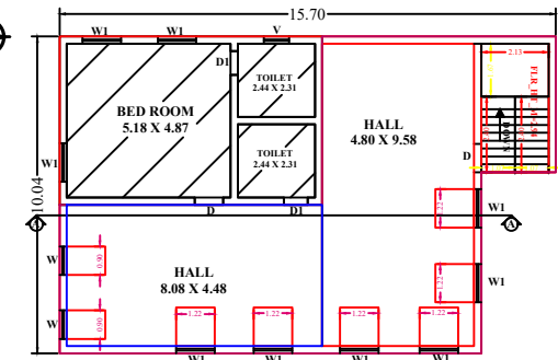
EXISTING & ADDITIONAL FIRST FLOOR PLAN
