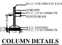
COLUMN DETAILS
