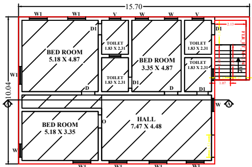
EXISTING GROUND FLOOR PLAN
