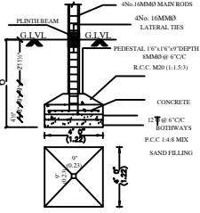
FOUNDATION DETAIL
