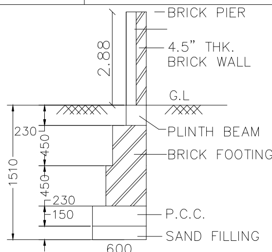
COMPOUND WALL DETAILS
