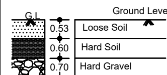
TRIAL PIT DETAILS (NOT TO SCALE)
