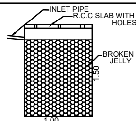
RAIN WATER HARVEST PIT
