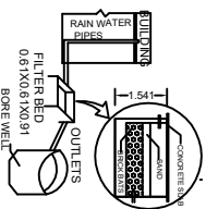
PLAN RAIN WATER HARVESTING SUMP
