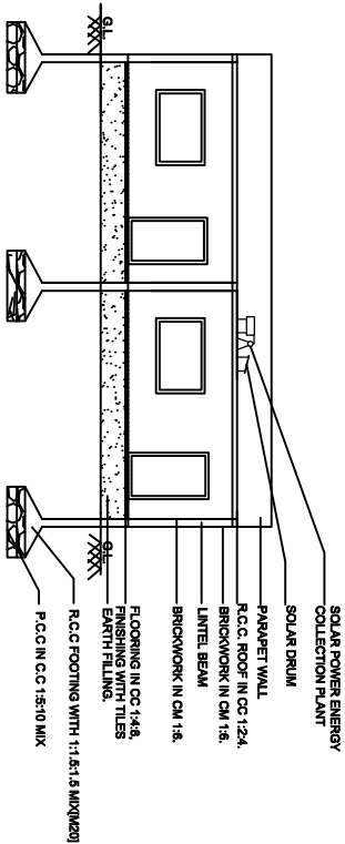
SECTION ON 'AB'
