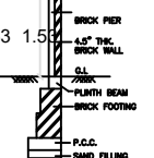
COMPOUND WALL
