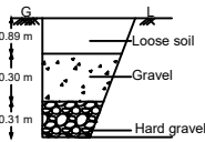
TRIAL PIT DETAILS (Not to Scale)
