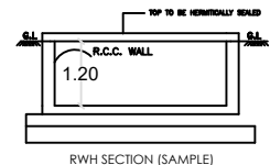
RWH_CAPACITY_L=2160LTRS
