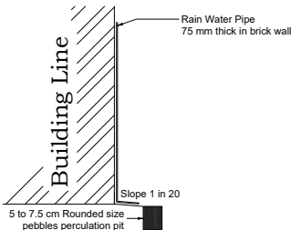
RAINWATER HARVESTING
