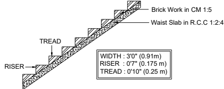
STAIRCASE DETAILS
