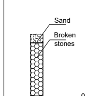
PERCOLATION PIT
