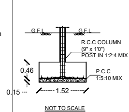
COLUMN POST DETAILS
