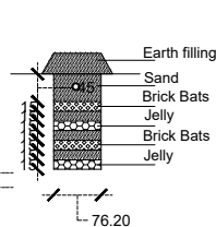
SECTION ON B-B.
