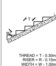
STAIRCASE DETAILS
