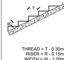
STAIRCASE DETAILS
